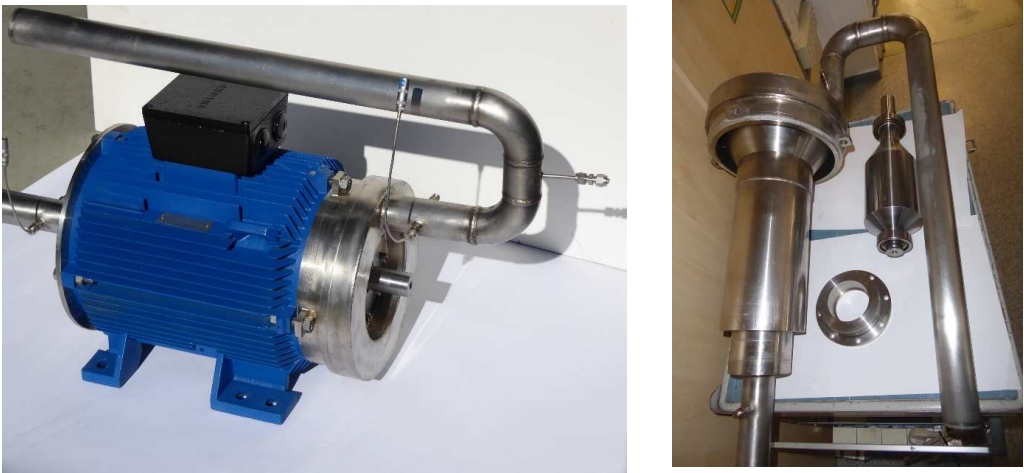
Fig. 4. Photograph of the assembled pump (left) and its components (right).
