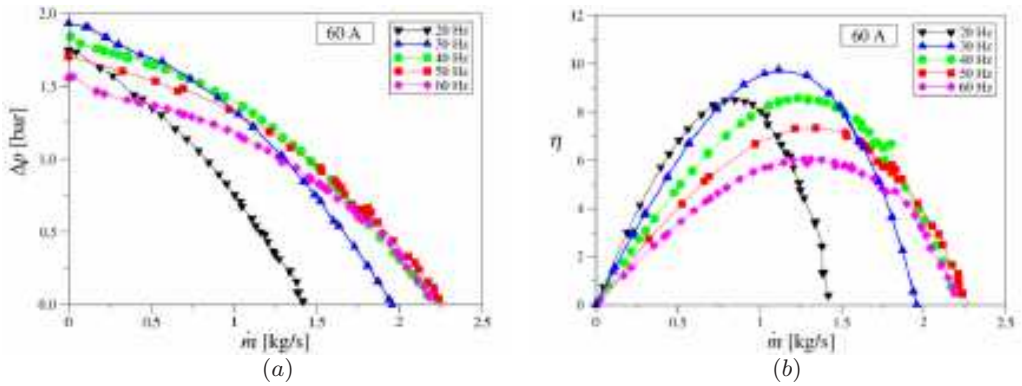
Fig. 5. Pressure head \Delta p (a) and efficiency \eta (b) versus mass flowrate \dot{m} for a total current I = 60 A and different frequencies.
